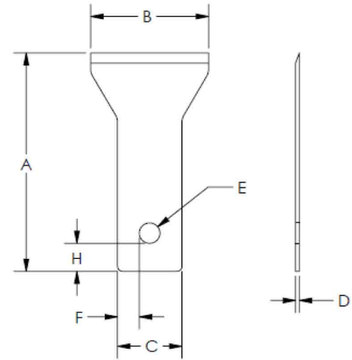
Single Bevel with Tapered ends
